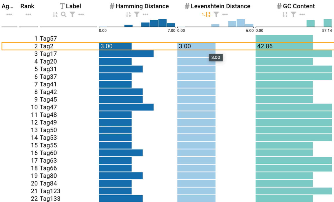
Fig. 4. Barcodes from Faircloth et al [43] with an active sort functionality on the Levenshtein column depicting the minimum distance and GC content.
