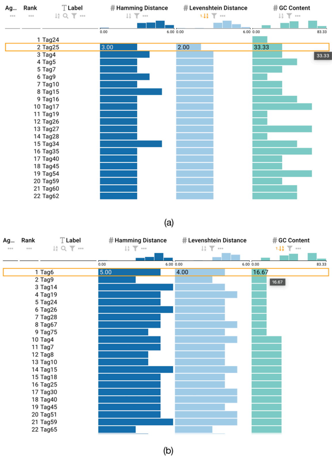
Fig. 6. Barcodes from Meyer et al. [42] with a selected sequence. (a) Active sort functionality on the Levenshtein column showing the minimum distance within the barcodes. (b) Active sort functionality on the GC content showing the lowest value.
