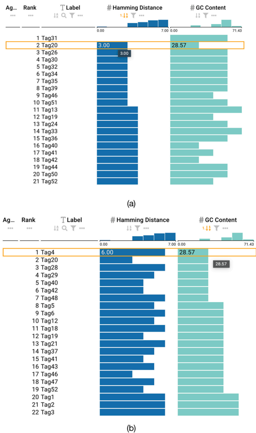
Fig. 7. Barcodes from Meyer et al. [45] based on Hamming distance with a selected sequence. (a) Active sort functionality on the Hamming column ranking the barcodes from smallest to largest. (b) Active sort functionality on the GC content showing the least GC content value.
