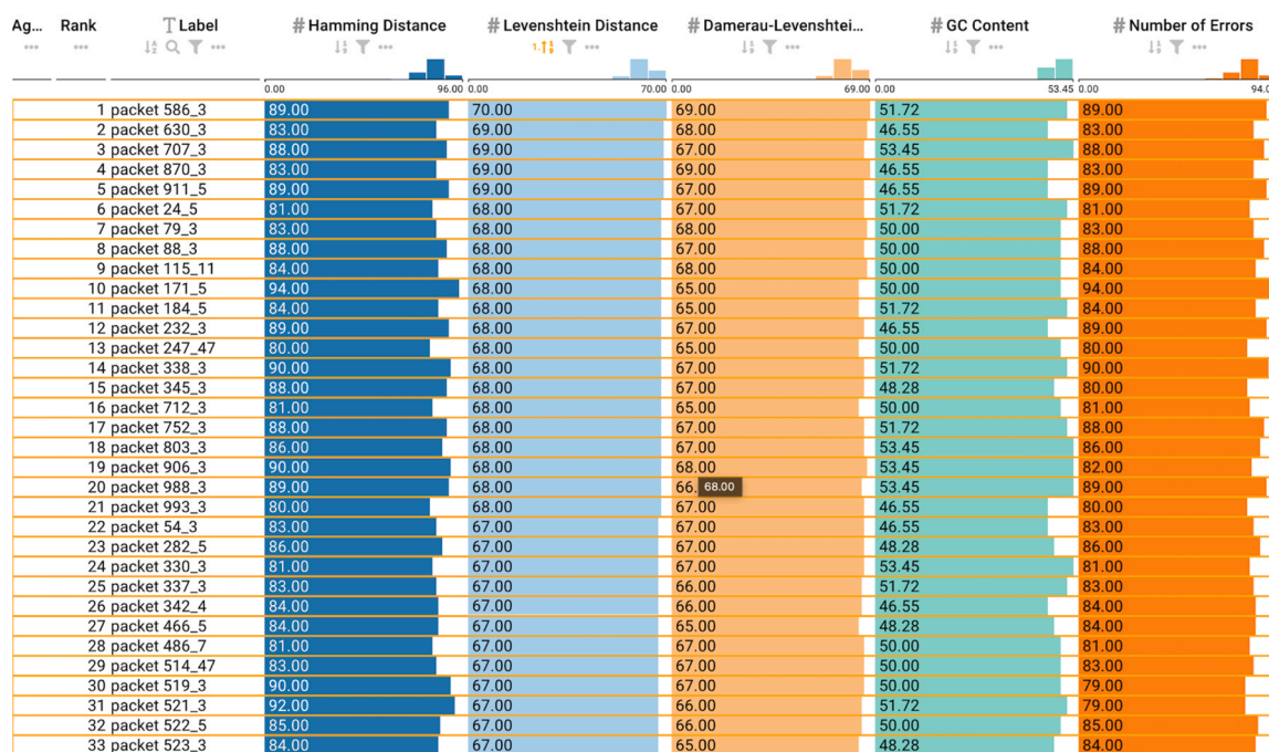
Fig. 9. Sequences from Fountain encoding scheme. Active sort functionality on the Levenshtein column. Selected sequences depict the ordering of sequences based on Levenshtein distance that is separated in the distance metric space.
