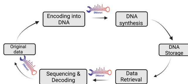
Fig. 1. Overview process of DNA data storage system with positions where DNAsmart can be used. DNAsmart accommodates sequences from either the synthesis or sequencing process.
