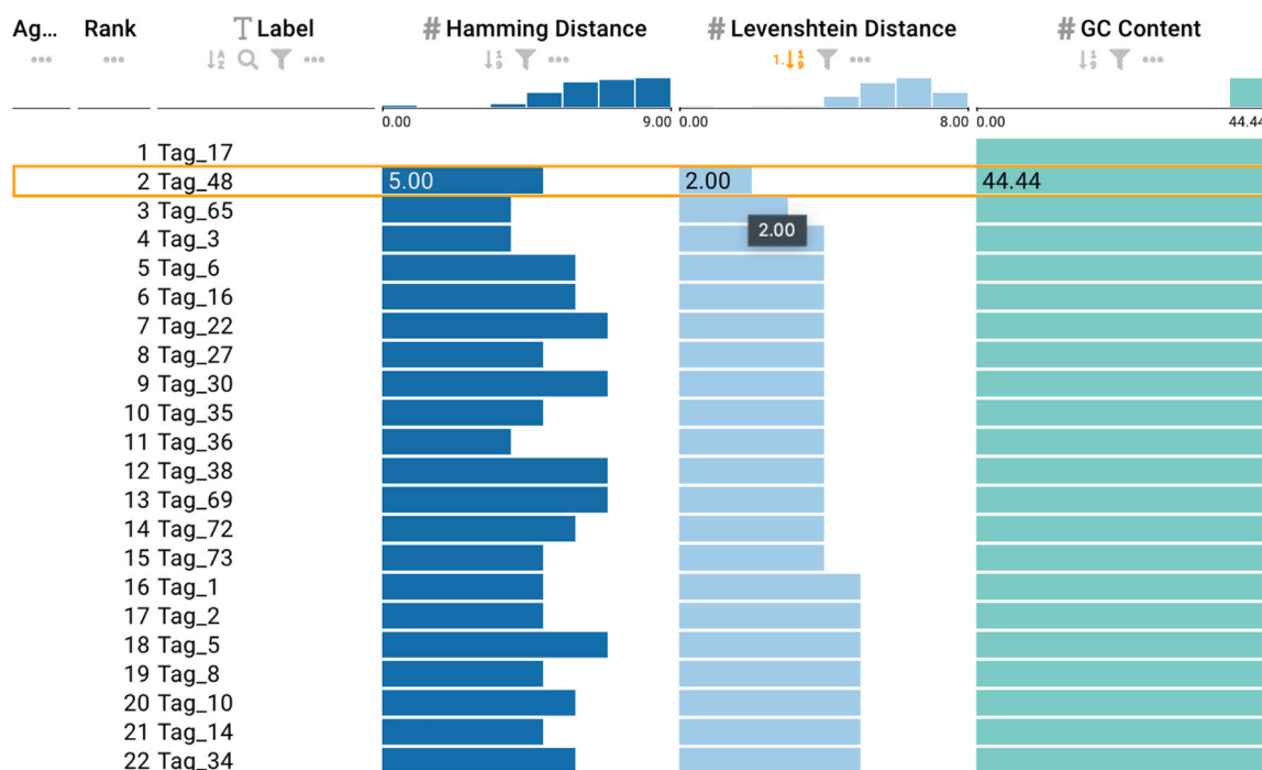
Fig. 5. Barcodes from Adey et al. [44] with an active sort functionality on the Levenshtein column depicting the minimum distance and GC content.
